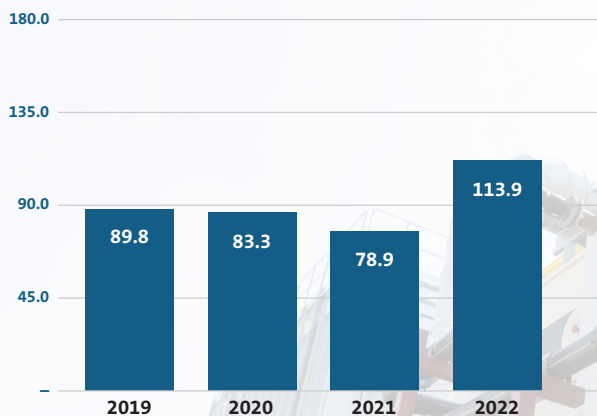
Hazardous Waste Disposal (Metric Tons) FY 2019-2022
