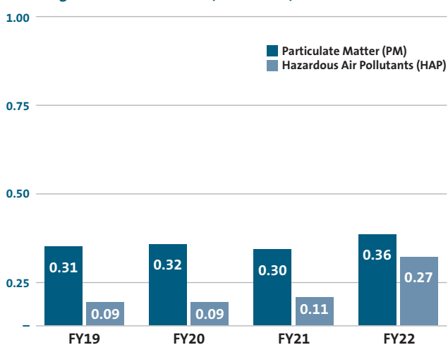
Other Significant Air Emissions (metric tons) FY 2019-2022
