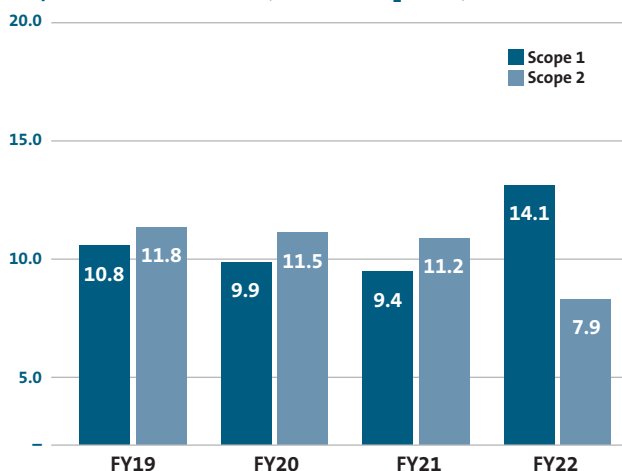
Scope 1 & 2 GHG Emissions (thousand CO 2 e Tons) FY 2019-2022
